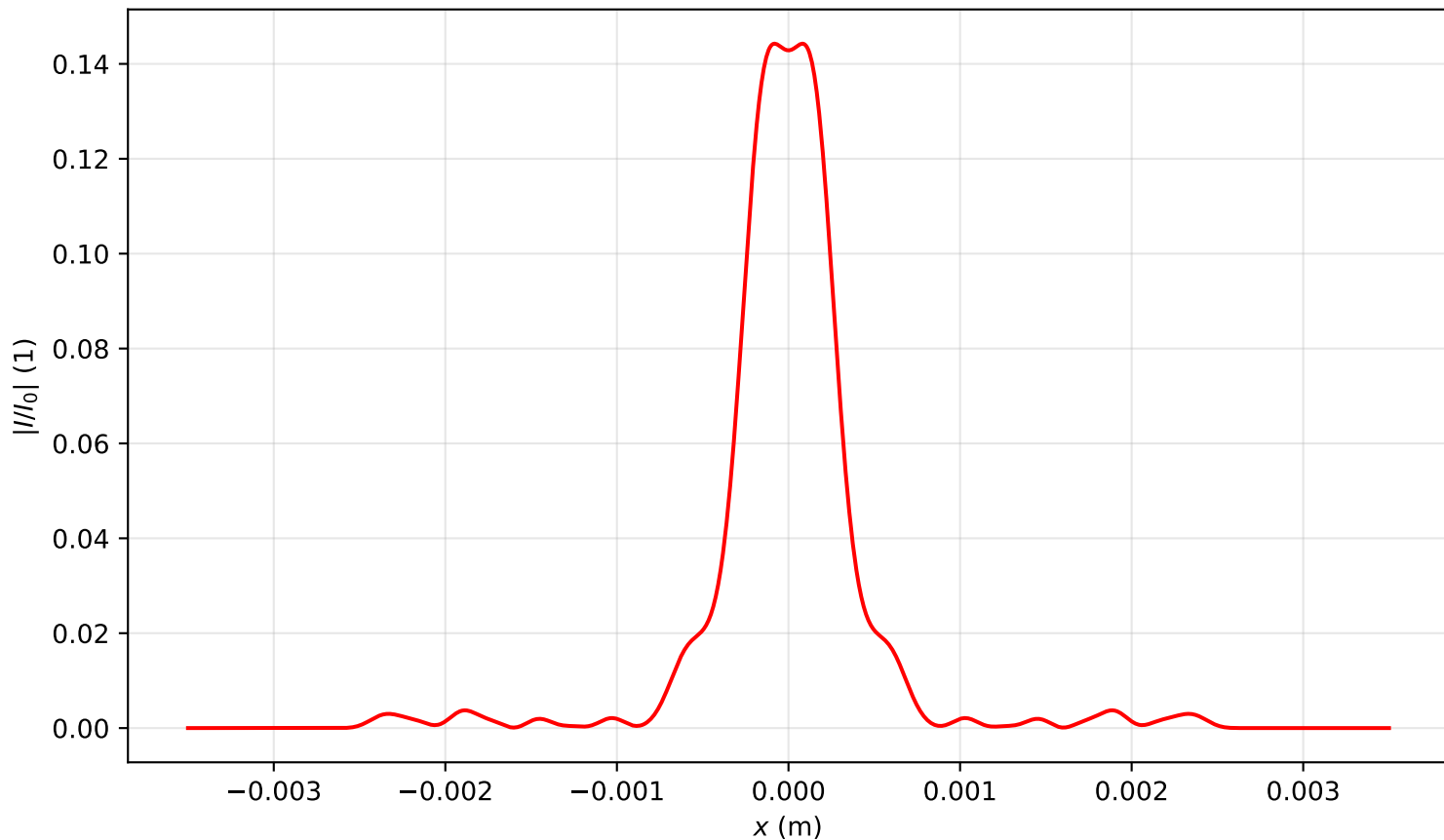
Intensity profile I(x, y = 0, z = 3.025)/I_0 , P_{in}=6.0P_{cr} , artificial time
